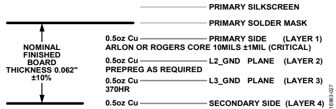
Figure 27. 4-Layer Stackup
