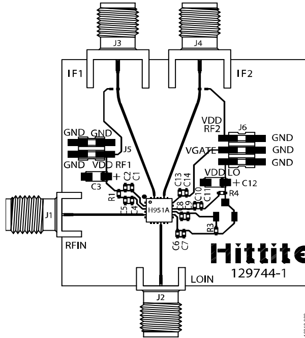
Figure 100. EV1HMC951ALP4 Evaluation Board Top Layer
