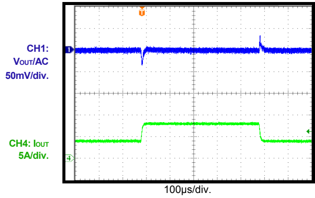
Transient Response
