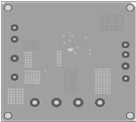
Figure 3— Inner 1 Layer
