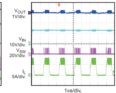
Short-Circuit Steady
