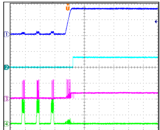
Short Circuit Protection Recovery
