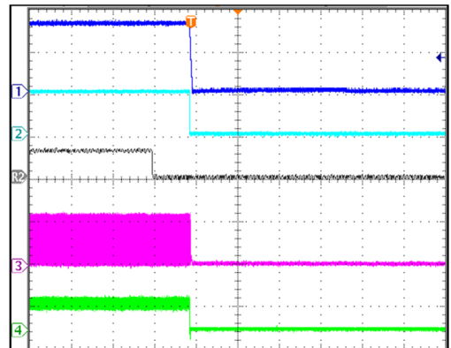
Short Circuit Protection Recovery
