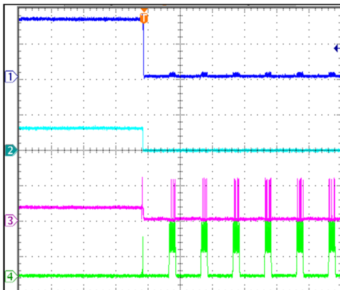
Short Circuit Protection Entry
