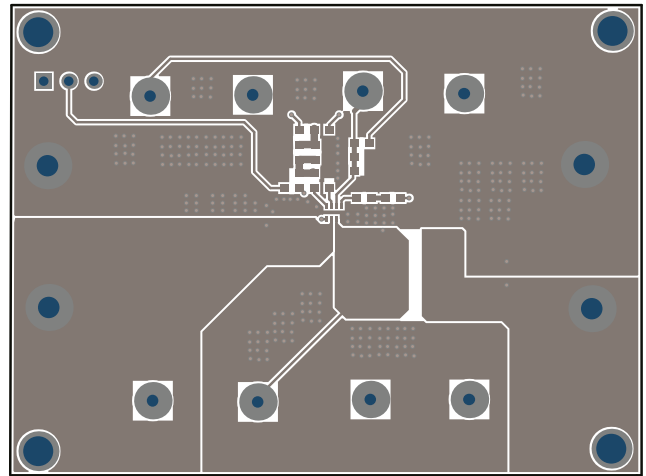
Figure 2: Top Layer
