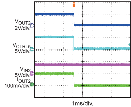
CTRL Off
