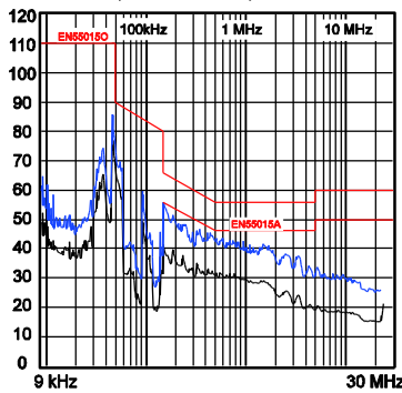
Conduction EMI
