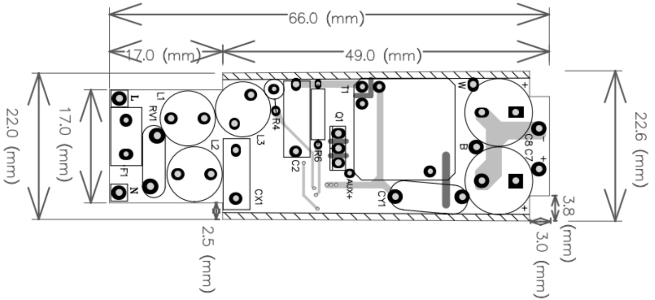
Figure 2 - Top Layer
