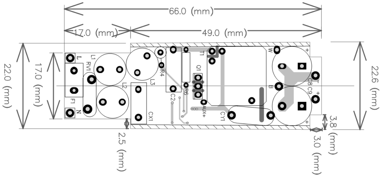
Figure 2 - Top Layer
