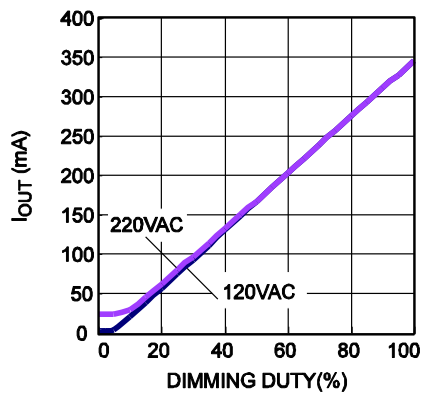
PWM Dimming Curve f_{PWM}=1kHz
