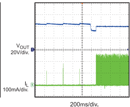
Open LED Protection Recovery
