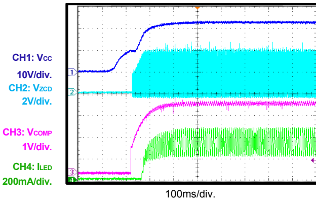
Start-Up V_{IN}=120Vac , 7 LED Output
