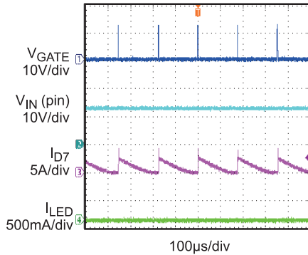
SCP steady state, LED+ short to LED- V_{AC}=220V
