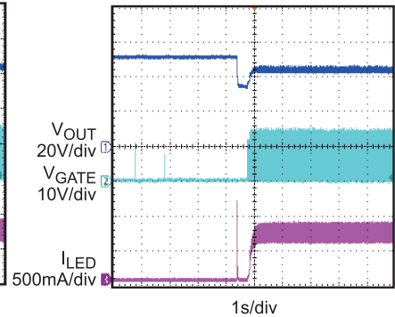
LED from open to full load V_{AC}=220V , full load
