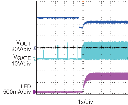
LED from open to full load V_{AC}=110V , full load
