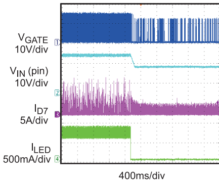
SCP entry, LED+ short to LED- V_{AC}=110V , full load
