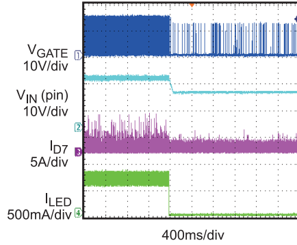
SCP entry, LED+ short to LED- V_{AC}=220V , full load
