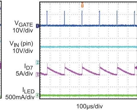
SCP steady state, LED+ short to LED- V_{AC}=110V
