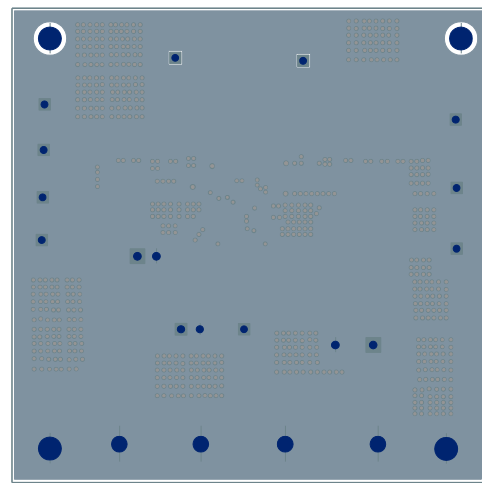
Figure 4—Mid 2 Layer
