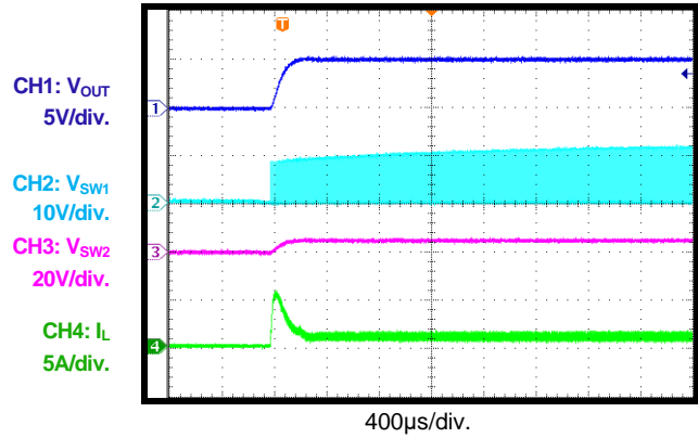
V_{IN} Start-Up Load = 1A
