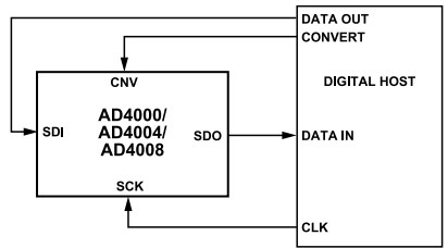
Figure 49. CS Mode, 3-Wire Turbo Mode Connection Diagram
