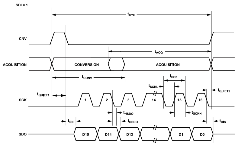
Figure 50. CS Mode, 3-Wire Turbo Mode Serial Interface Timing Diagram (Status Bits Not Shown)
