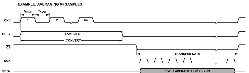
Figure 54. Example Conversion Cycle for Averaging Mode
