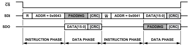
Figure 92. Single Instruction Mode SPI Frame, MB_STRICT = 1, Descending Address
