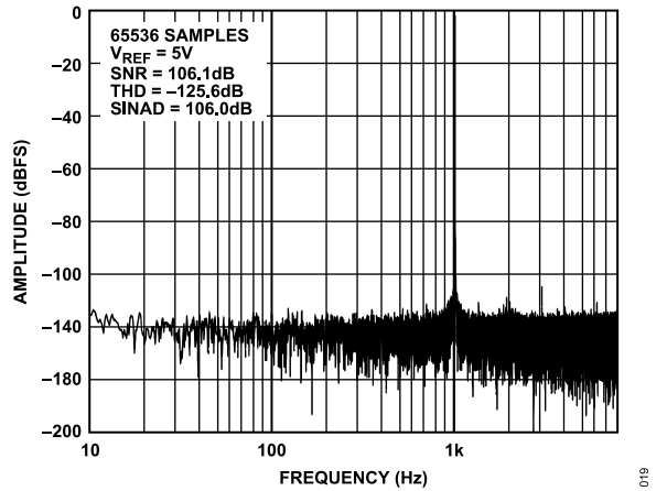
Figure 20. FFT, f_{IN} = 1 kHz, V_{REF} = 2.5 V, OSR = 64
