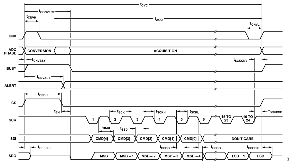
Figure 96. Conversion Mode Timing Diagram, Single-SDO Mode, SDO_STATE = 1
