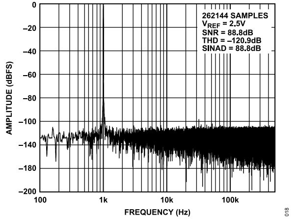
Figure 19. FFT, f_{IN} = 1 kHz, V_{REF} = 2.5 V, OSR = 1
