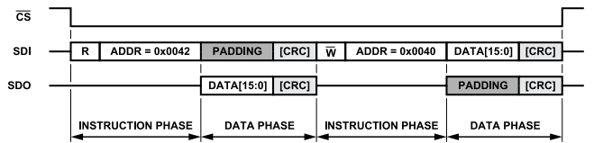
Figure 93. Single Instruction Mode SPI Frame, MB_STRICT = 1, Ascending Address
