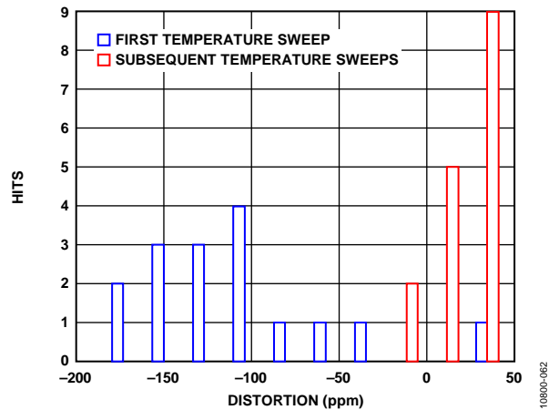
Figure 50. Thermal Hysteresis
