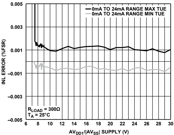
Figure 42. INL Error vs. AV_{DD1}/AV_{SS} Supply, External R_{SET}
