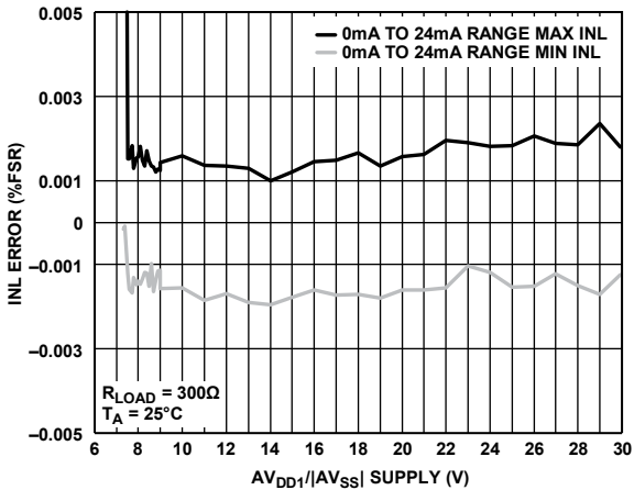
Figure 41. INL Error vs. AV_{DD1}/AV_{SS} Supply, Internal R_{SET}
