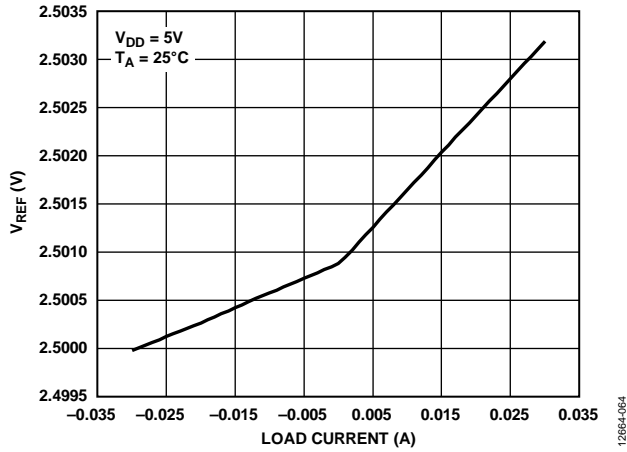
Figure 53. V_{REF} vs. Load Current and V_{DD}
