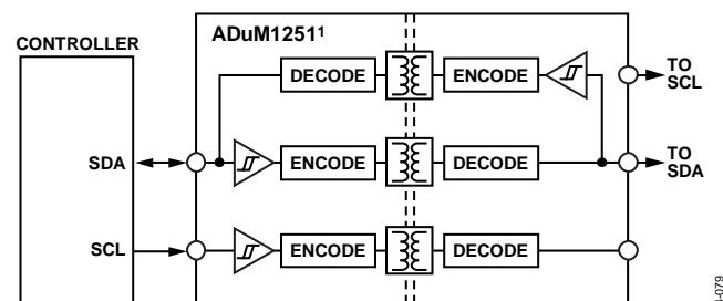
Figure 69. Isolated Interface
