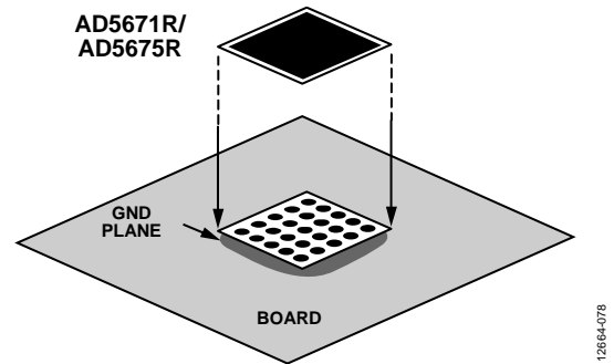
Figure 68. Pad Connection to Board
