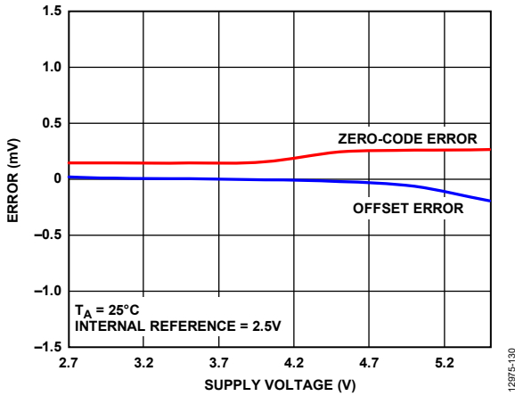
Figure 27. Zero-Code Error and Offset Error vs. Supply
