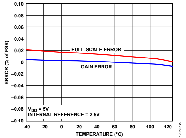
Figure 24. Gain Error and Full-Scale Error vs. Temperature
