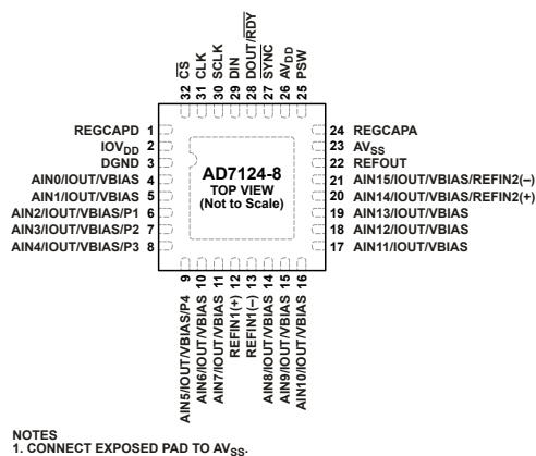
Figure 9. Pin Configuration
