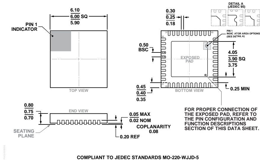
Figure 75. 40-Lead Lead Frame Chip Scale Package [LFCSP] 6 mm × 6 mm Body and 0.75 mm Package Height (CP-40-14) Dimensions shown in millimeters
