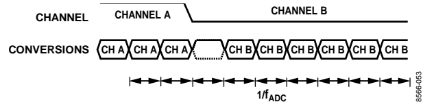
Figure 54. Fast Settling, Sinc 4 Filter
