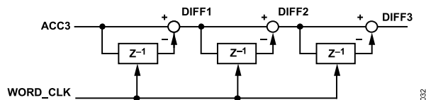
Figure 38. Differentiator
