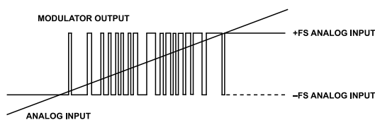
Figure 28. Analog Input vs. Modulator Output
