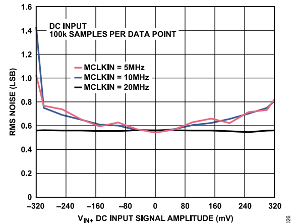
Figure 32. RMS Noise vs. V_{IN+} DC Input Signal Amplitude
