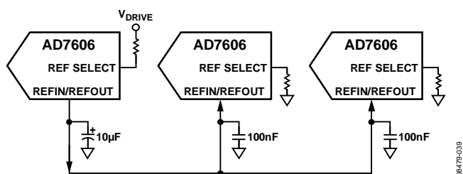
Figure 42. Internal Reference Driving Multiple AD7606/AD7606-6/AD7606-4 REF IN Pins
