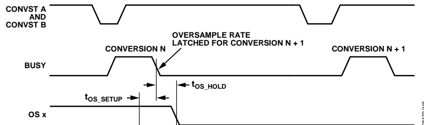
Figure 48. OS x Pin Timing
