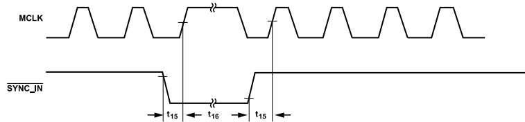
Figure 6. Synchronous SYNC_IN Pulse Timing Diagram
