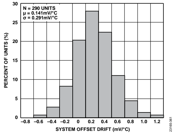
Figure 66. System Offset Drift Distribution, T_z = 200\text{ k}\Omega , LPF = 1 MHz
