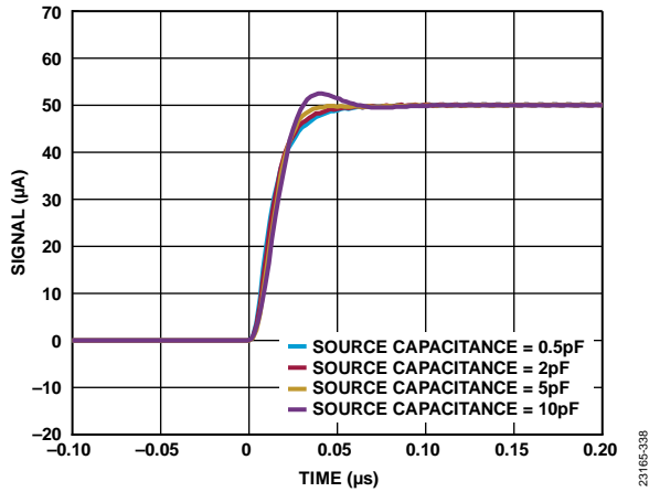
Figure 38. Pulse Response Rising Edge for Various Source Capacitances, T_z = 20\text{ k}\Omega , LPF = 100\text{ MHz}
