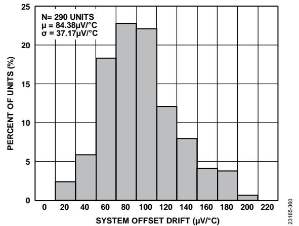
Figure 65. System Offset Drift Distribution, T_z = 20\text{ k}\Omega , LPF = 100 MHz
