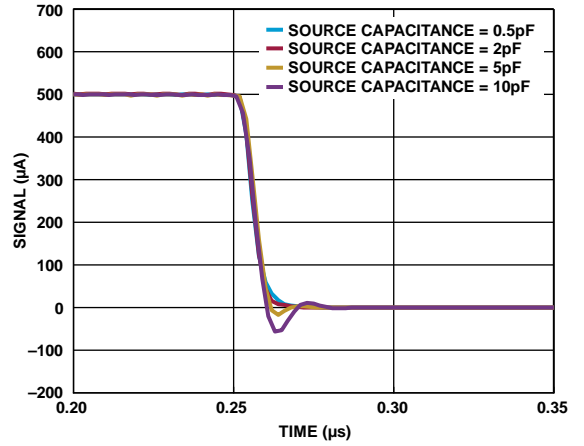
Figure 40. Pulse Response Falling Edge for Various Source Capacitances, T_z = 2\text{ k}\Omega , LPF = 100\text{ MHz}
