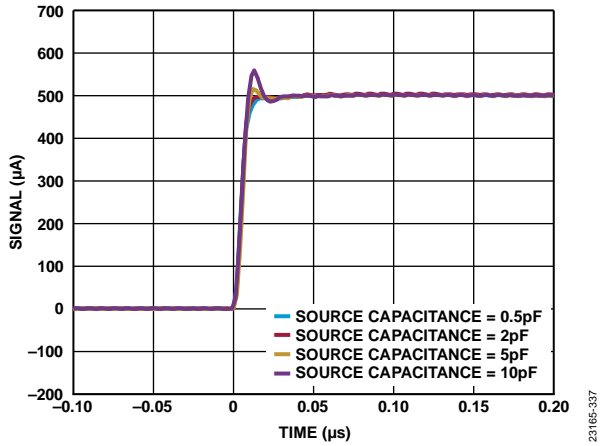
Figure 37. Pulse Response Rising Edge for Various Source Capacitances, T_z = 2\text{ k}\Omega , LPF = 100\text{ MHz}
