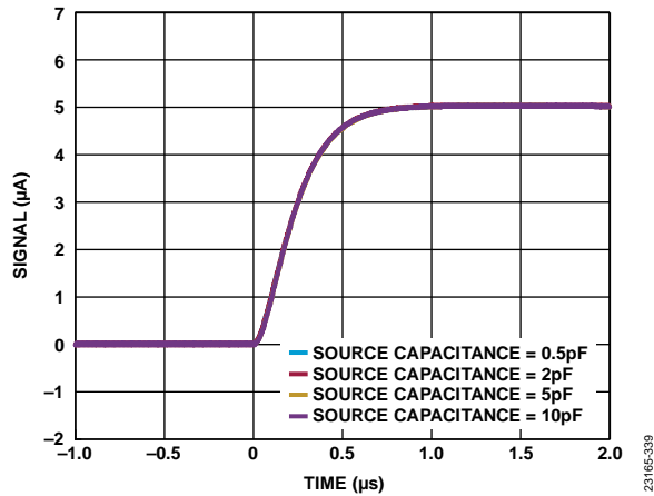
Figure 39. Pulse Response Rising Edge for Various Source Capacitances, T_z = 200\text{ k}\Omega , LPF = 1\text{ MHz}
