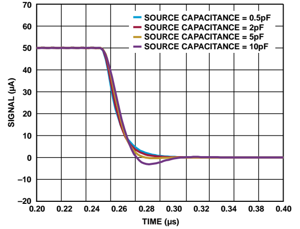
Figure 41. Pulse Response Falling Edge for Various Source Capacitances, T_z = 20\text{ k}\Omega , LPF = 100\text{ MHz}
