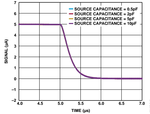
Figure 42. Pulse Response Falling Edge for Various Source Capacitances, T_z = 200\text{ k}\Omega , LPF = 1\text{ MHz}
