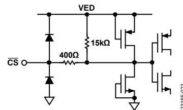
Figure 76. Equivalent CS-bar Input Circuit
