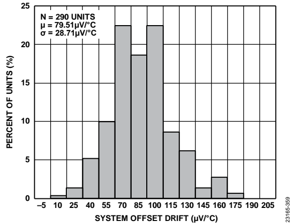
Figure 64. System Offset Drift Distribution, T_z = 2\text{ k}\Omega , LPF = 100 MHz
