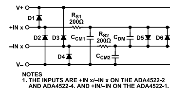
Figure 72. Input EMI Filter and Clamp Circuit
