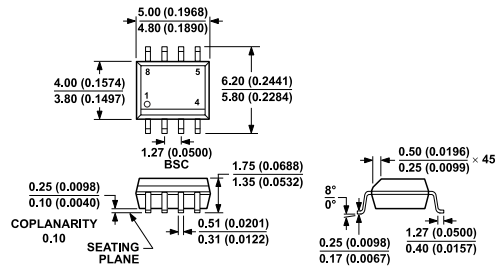
Figure 91. 8-Lead Small Outline Package [SOIC_N] Narrow Body (R-8) Dimensions shown in millimeters and (inches)
