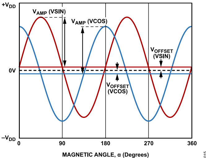
Figure 15. Differential Output Voltage Range
