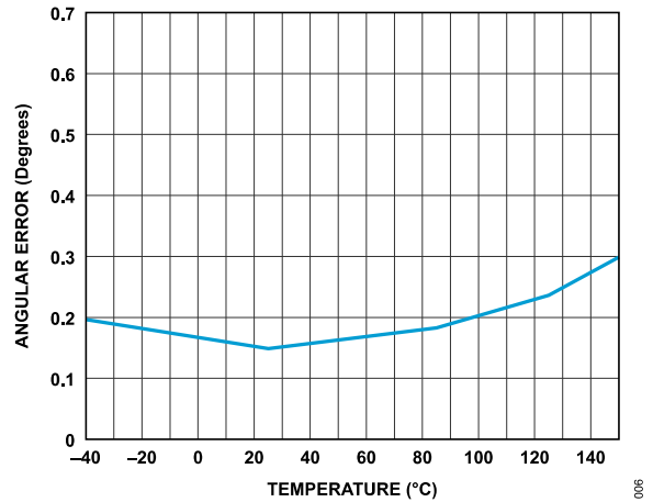
Figure 6. Single Point Calibration Angular Error vs. Temperature
