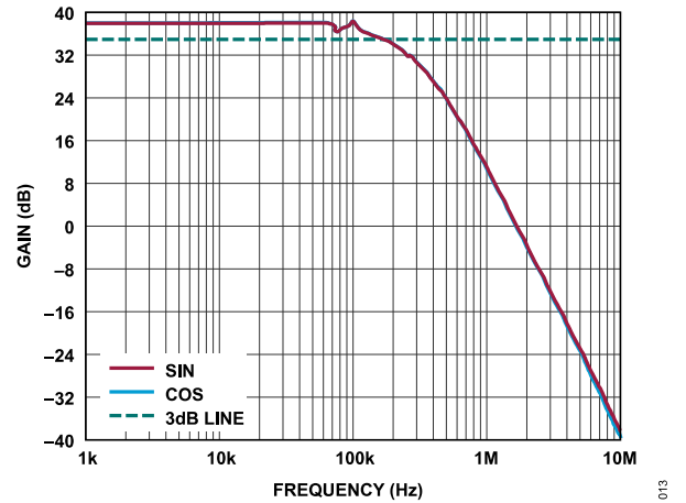
Figure 13. Frequency Response
