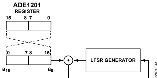
Figure 42. CRC Calculation
