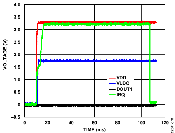
Figure 14. Power-Up of Nonisolated Side (VDD, VLDO, DOUT1, and \overline{\text{IRQ}} Pins)
