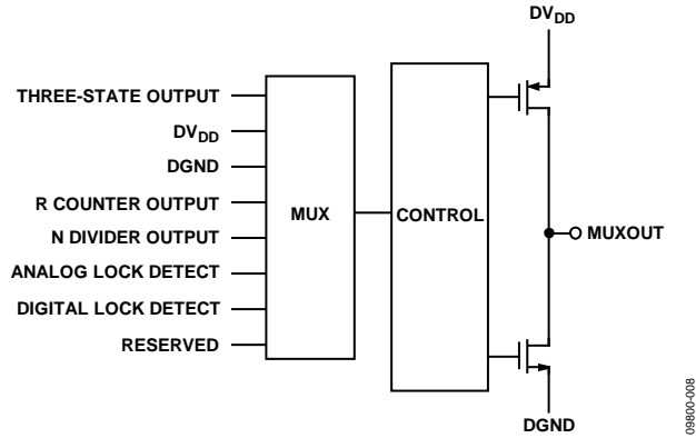
Figure 19. MUXOUT Schematic
