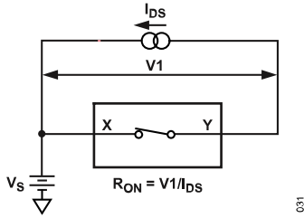
Figure 25. On Resistance
