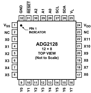
Figure 3. Pin Configuration
