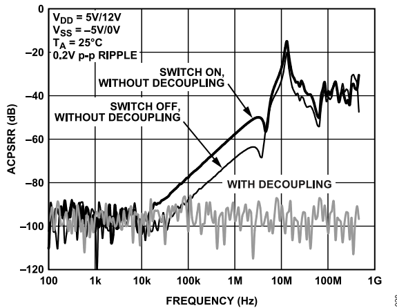
Figure 24. ACPSRR
