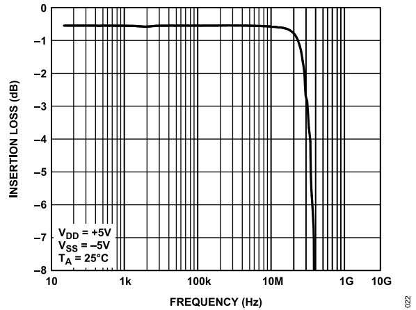
Figure 19. One Input to Eight Outputs Bandwidth, 5 V Dual Supply
