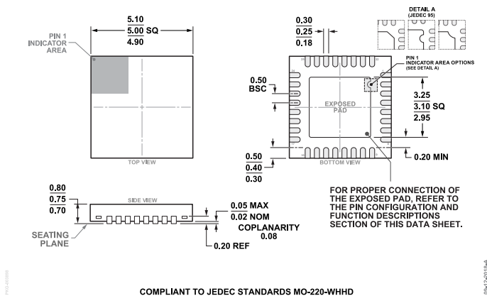
Figure 38. 32-Lead Lead Frame Chip Scale Package [LFCSP] 5 x 5 mm Body and 0.75 mm Package Height (CP-32-7) Dimensions shown in millimeters
