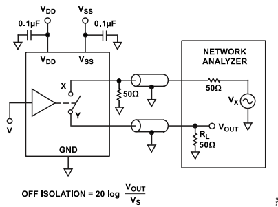
Figure 30. Off Isolation
