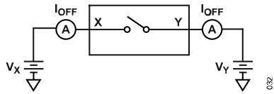
Figure 26. Off Leakage
