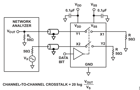
Figure 32. Channel-to-Channel Crosstalk
