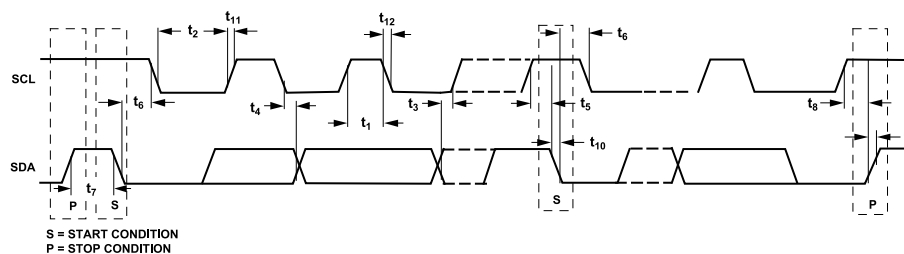
Figure 2. Timing Diagram for 2-Wire Serial Interface
