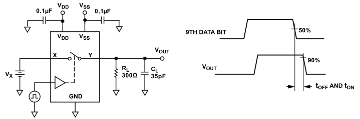
Figure 28. Switching Times, tON, tOFF
