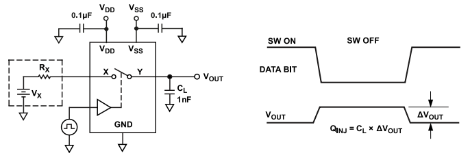
Figure 29. Charge Injection
