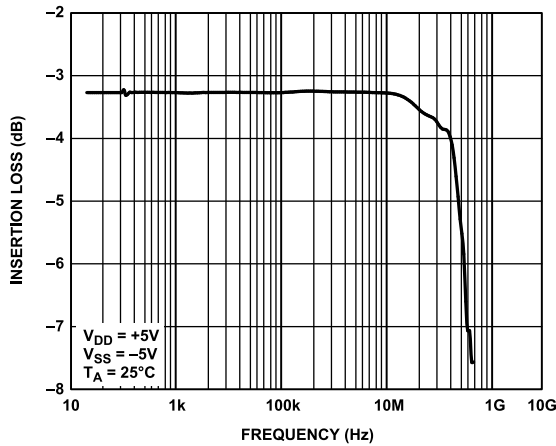
Figure 17. Individual Inputs to Individual Outputs Bandwidth, Dual \pm 5 V Supply
