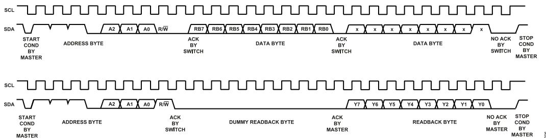
Figure 35. Read Operation
