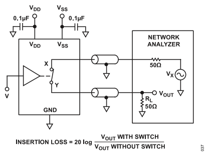
Figure 31. Bandwidth
