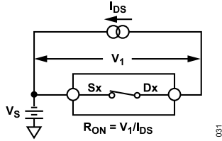
Figure 31. On Resistance
