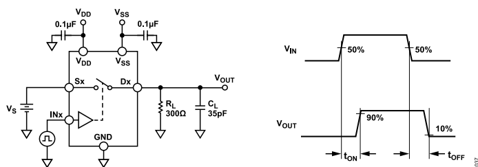
Figure 37. Switching Times
