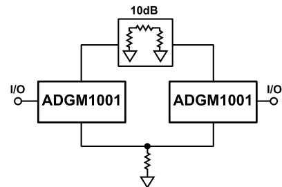
Figure 59. Switching RF Attenuators Using ADGM1001 MEMS Switches
