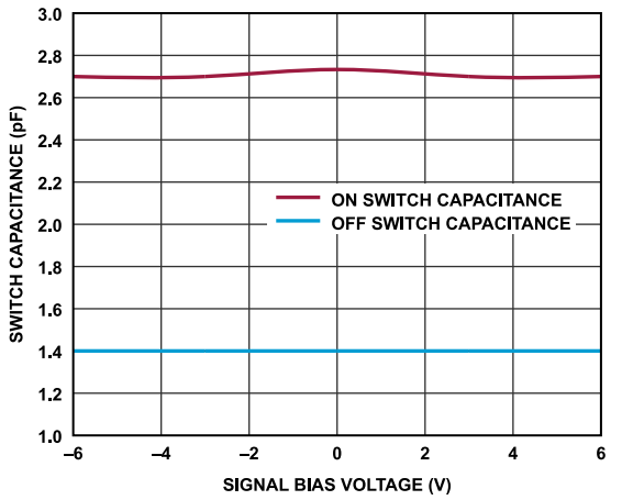
Figure 38. Switch Capacitance vs. Signal Bias Voltage
