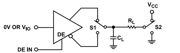
Figure 40. Driver Propagation Delay
