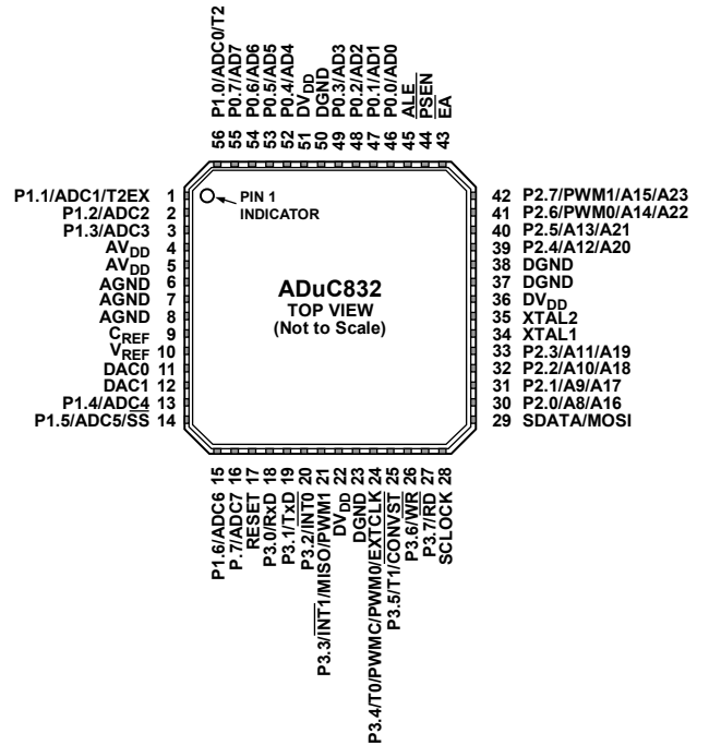
Figure 15. 56-Lead LFCSP
