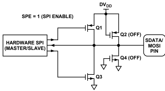
Figure 73. SDATA/MOSI Pin I/O Functional Equivalent in SPI Mode
