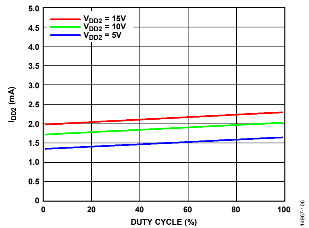
Figure 9. I_{DD2} vs. Duty Cycle, V_{DD1} = 5\text{ V} , Switching Frequency ( f_{sw} ) = 10 kHz, 2 nF Load
