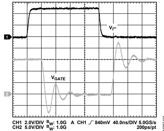
Figure 7. V_{I-} to V_{GATE} Waveform for 2 nF Load, 0 Ω Series Gate Resistor, V_{DD2} = 15\text{ V}
