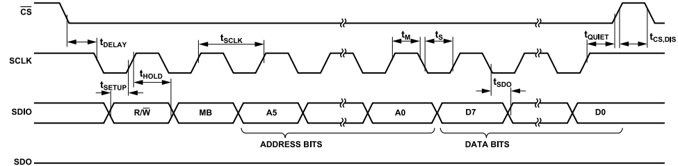
Figure 27. SPI 3-Wire Read/Write
