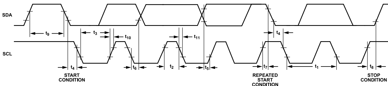
Figure 23. I 2 C Timing Diagram
