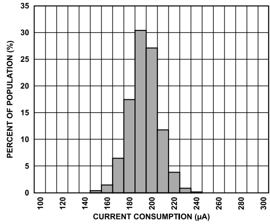
Figure 14. Current Consumption, Measurement Mode, Data Rate = 100 Hz, V_S = V_{DD I/O} = 3.3 V, 25^\circ C
