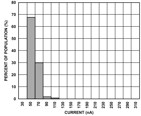
Figure 13. Standby Mode Current Consumption, V_S = V_{DD I/O} = 3.3 V, 25^\circ C
