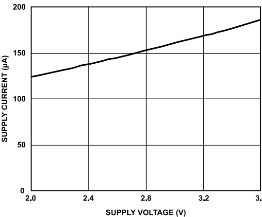
Figure 15. Supply Current vs. Supply Voltage, V_S at 25^\circ C
