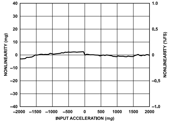
Figure 7. X-Axis Nonlinearity, \pm 2 g Input Range
