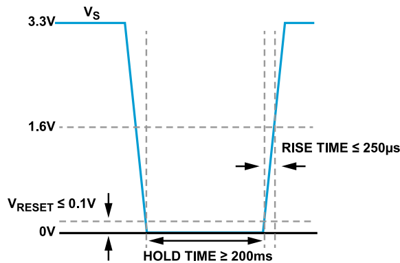
Figure 48. Power Cycling Requirements
