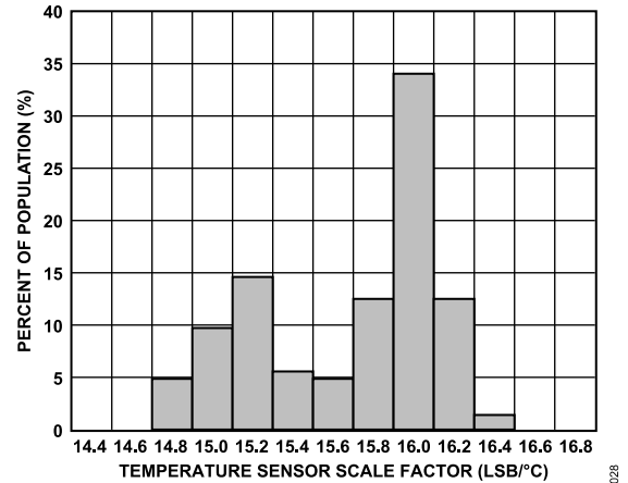
Figure 28. Temperature Sensor Scale Factor, V_S = 2 V
