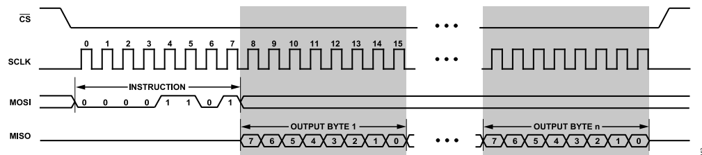
Figure 40. FIFO Read
