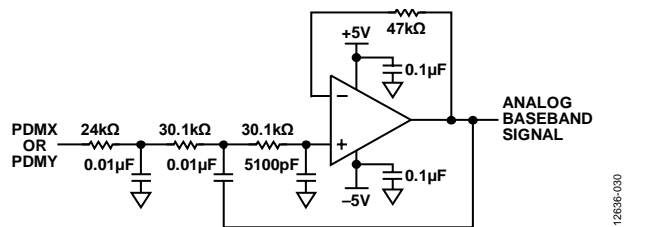
Figure 28. Recommended Low-Pass Filter for Demodulating the PDM Output in Analog Mode Operation
