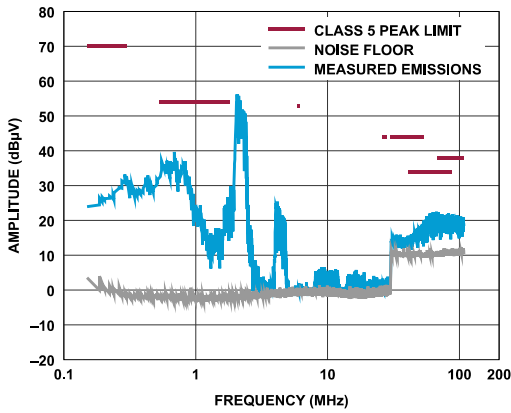
Figure 5. Peak Conducted Emissions (Voltage Method)
