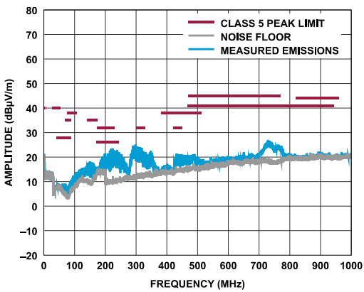
Figure 7. Peak Radiated Emissions (ALSE Method)
