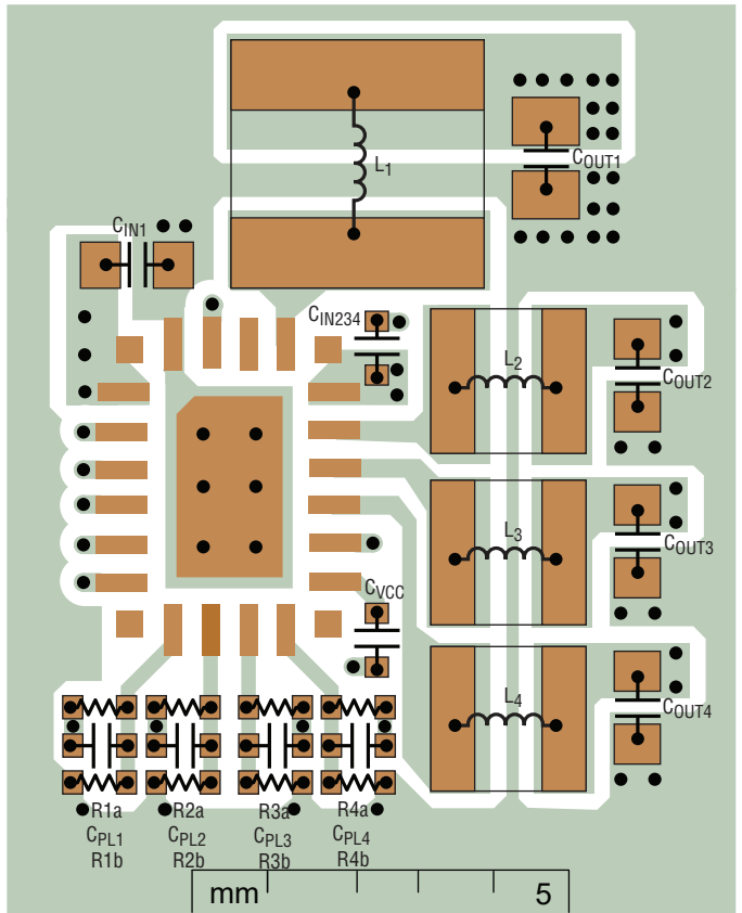
Figure 7. Smallest Layout
