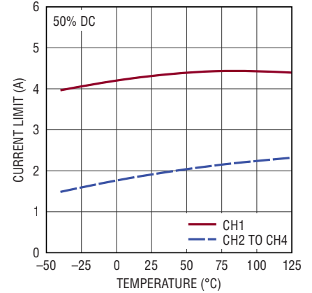
Top MOSFET Current Limit
