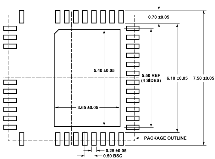
Figure 37. 48(39)-Lead Plastic QFN (7 mm × 7 mm) (05-08-1792)
