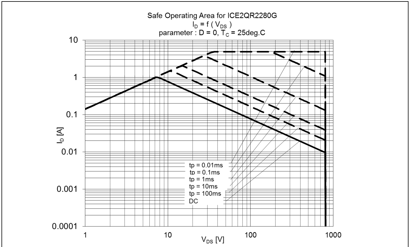
Figure 10 Safe Operating Area (SOA) curve for ICE2QR2280G
