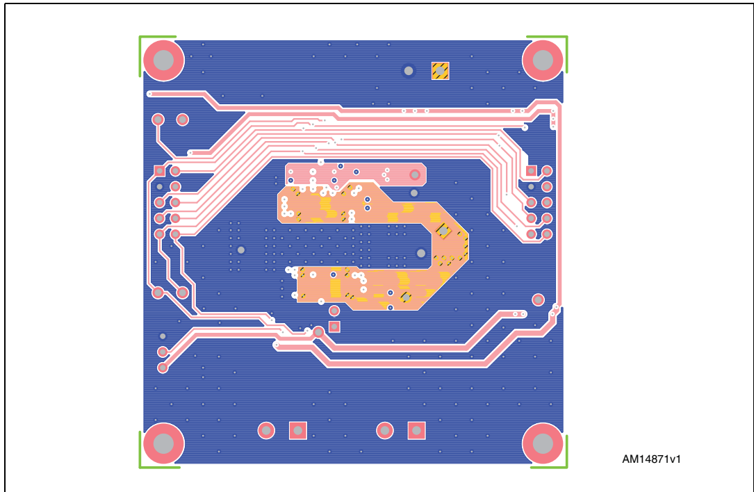
Figure 6. EVAL6474PD - layout (bottom layer3)
