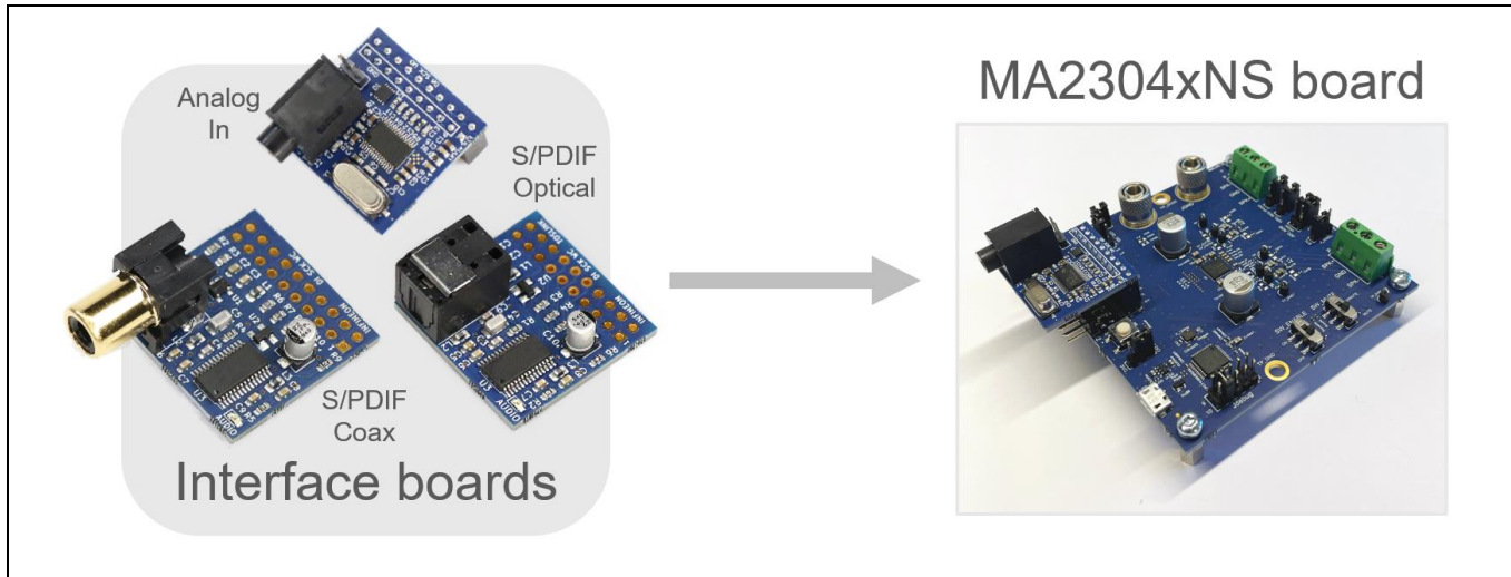
Figure 3 Interface boards
