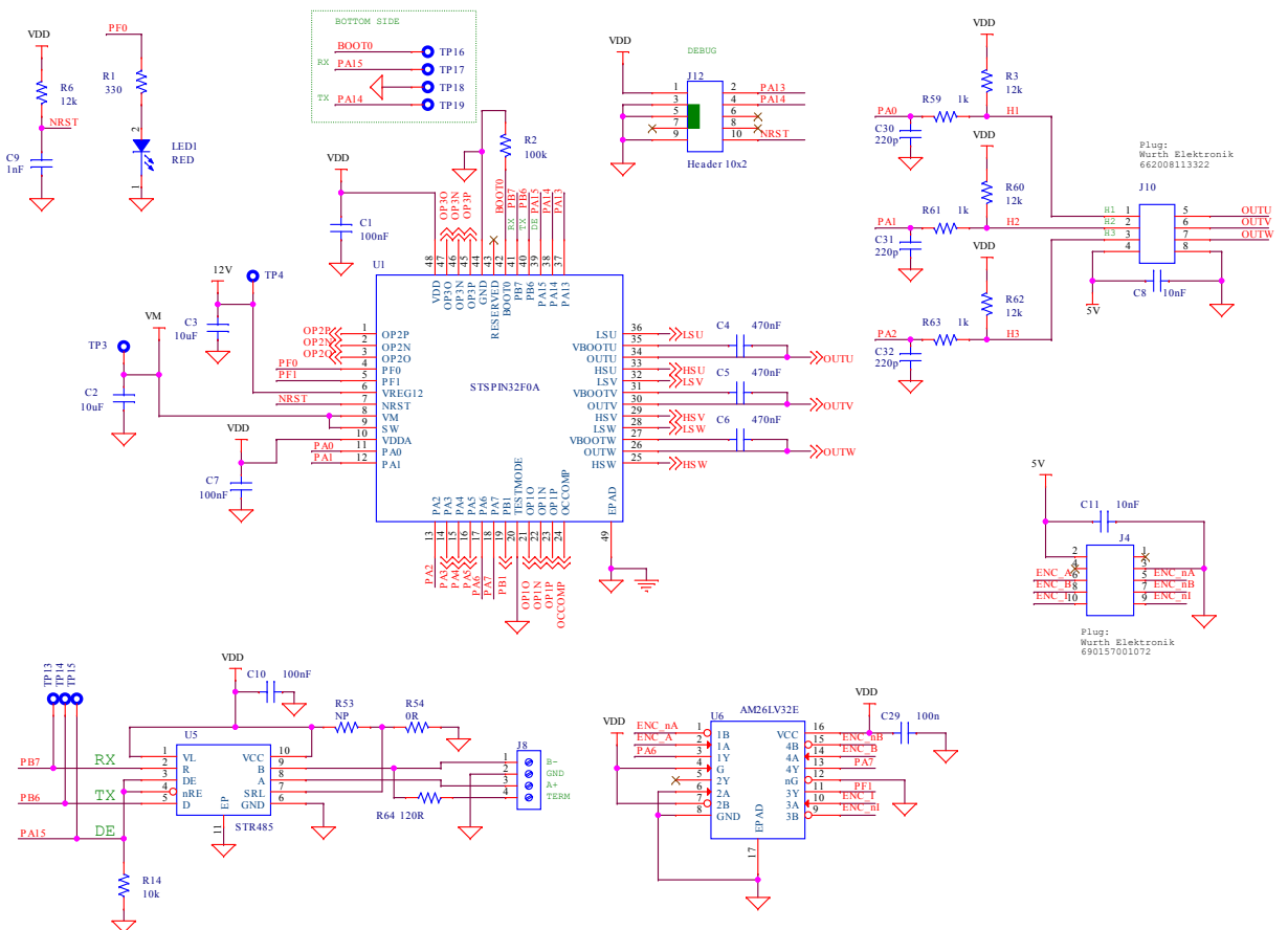
Figure 3. Schematic board 1
