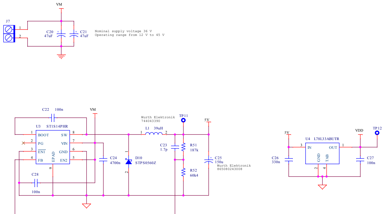
Figure 5. Schematic board 3
