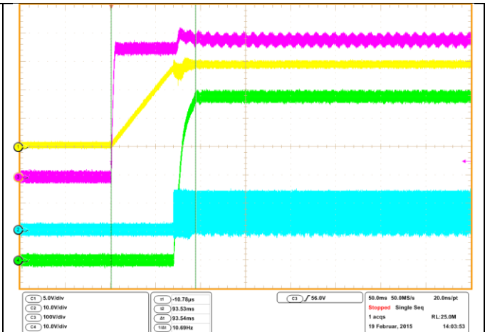
Figure 9: AC Input Voltage 300V ACIN , Full Load
